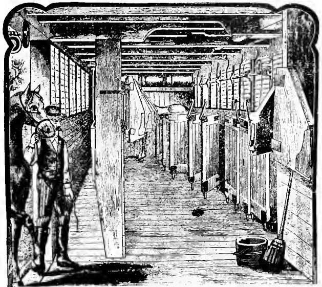
Fig. 43. INTERIOR OF STOCK CAR FOR HORSES. KEYSTONE PALACE HORSE CAR COMPANY. Capacity, 18 horses.
